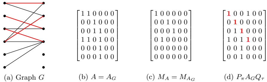
Fig. 1: Then, \pi is the identity permutation, and \tau fixes 1, moves 2 to 4, 3 to 2, 4 to 3, and fixes 5 and 6. The lines in red in (a) indicate a maximal matching; the red ones in (d) indicate the corresponding lines, now placed on diagonal. Note that the 2 \times 2 lower-right submatrix is zero as it should.
