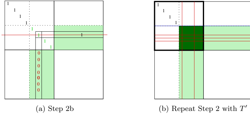
Fig. 2: In (b), T' is the upper-left quadrant, emphasized with a thicker border, with the “green square” zeroed out, as well as the entries under the red lines, arising from the cover of the “green square,” zeroed out.
